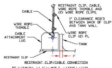
RESTRAINT CLIP/CABLE CONNECTION
