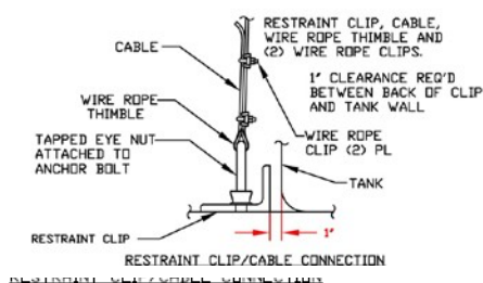
RESTRAINT CLIP/CABLE CONNECTION
